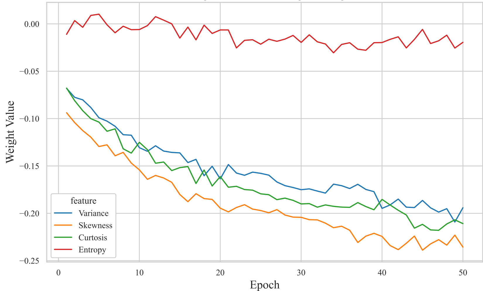
Weight Evolution During Training
